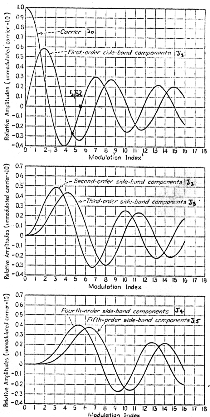
Fig. 2. Bessel functions which determine the amplitudes of the sideband components.
