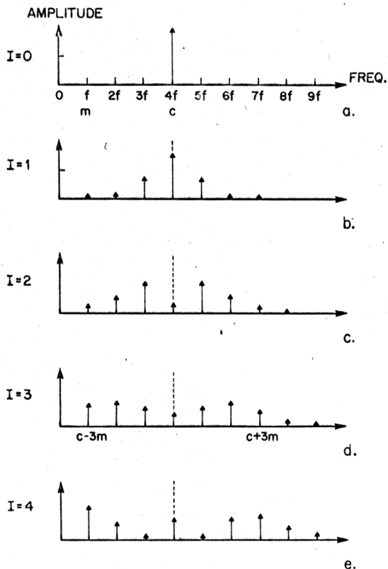
Fig. 5. Plot of spectrum where the ratio of c/m is 4/1 . As the index increases, the reflected lower side frequencies begin to affect the spectrum when I = 3 , where the fundamental, c-3m , is noticeably greater than the 7th harmonic, c+3m . In e, the symmetry around the carrier is no longer apparent.
