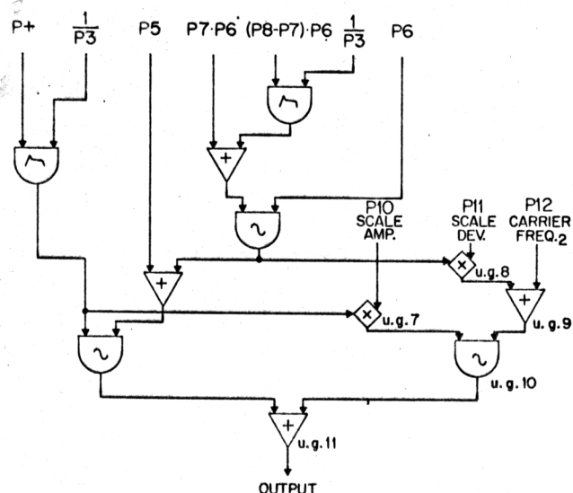
Fig. 17. FM circuit which allows greater control over the spectrum. The additional carrier wave uses the same modulating wave but the deviation can be scaled up or down by the multiplier. A formant peak can be placed at an arbitrary point in the spectrum.
