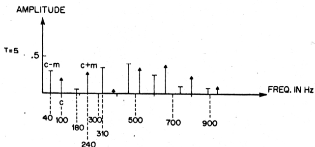
Fig. 6. Inharmonic spectrum where the ratio c/m \approx 1/\sqrt{2} and the modulation index = 5 . The reflected components, represented here with the bar at the top, fall in between the other components.
