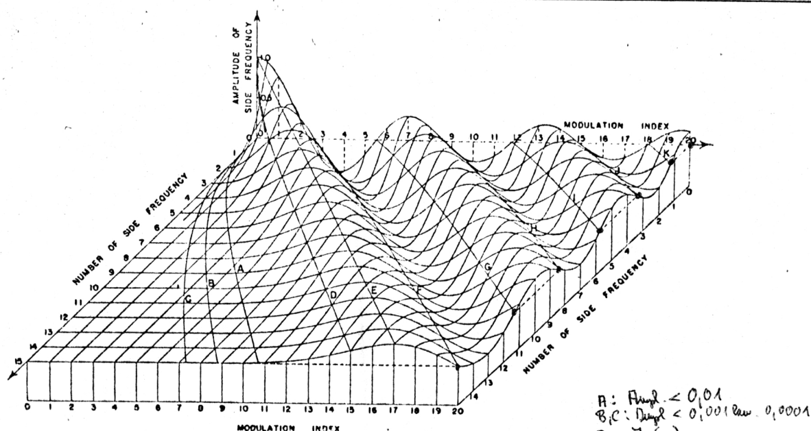
Fig. 8. Bessel functions, J_n through J_{15} and indexes 0 through 20. This representation allows a rapid determination of the bandwidth resulting from a given index.
