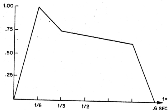
Fig. 11. Envelope function for brass-like tones.
