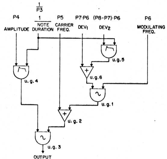
Fig. 10. FM circuit to produce dynamic spectra. Two function generators are added, u.g. 4 and u.g. 5, to produce an amplitude envelope and a modulation index envelope which causes the bandwidth to vary.
