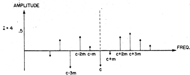
Fig. 3. Plot of Fig. 1e with phase information included (modulation index = 4). The bars extending downward represent spectral components whose phases differ by 180°.
