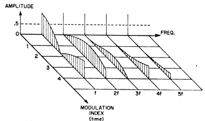
Fig. 7. Dynamic spectrum where the ratio c/m = 1/1 and the modulation index increases from 0 to 4 continuously. The increasing bandwidth is easily seen, but because the spectrum includes the reflected side frequencies, the evolution of the individual components is not always intuitively clear.
